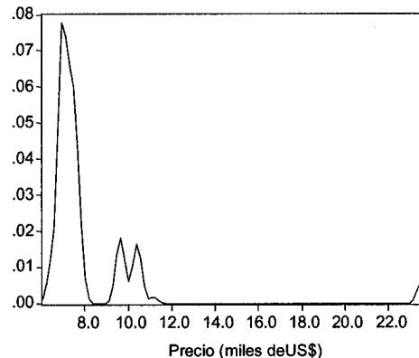
Kernel Density (Normal, h = 2.5476 )
