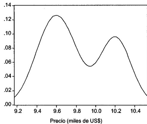
Tailandia Kernel Density (Normal, h = 1.6287 )
