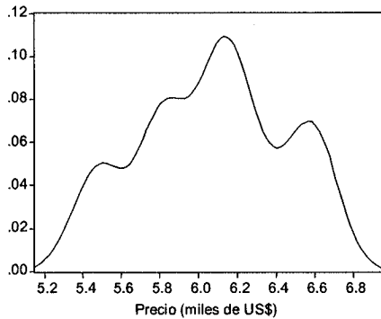
Kernel Density (Normal, h = 2.5476 )
