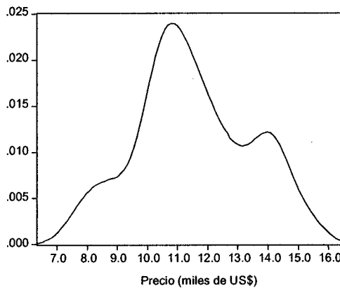
Kernel Density (Normal, h = 4.8207 )
