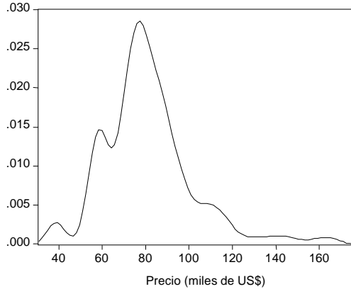
Kernel Density (Normal, h = 4.1176 )
