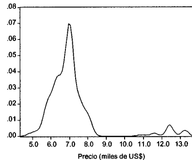
Kernel Density (Normal, h = 2.7217 )
