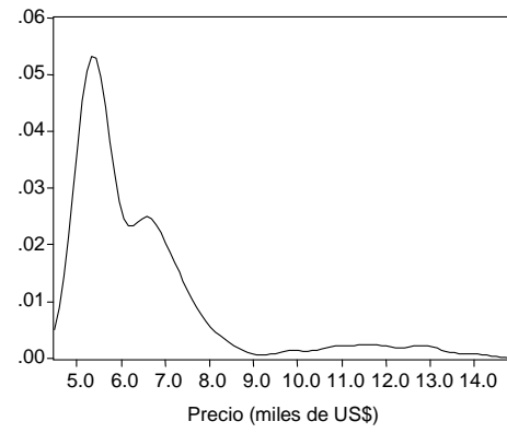
Kernel Density (Normal, h = 2.8788 )
