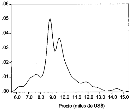
Kernel Density (Normal, h = 2.6707 )
