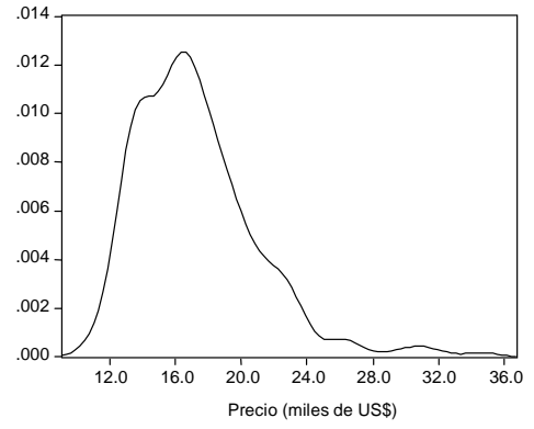
Kernel Density (Normal, h = 9.2715 )
