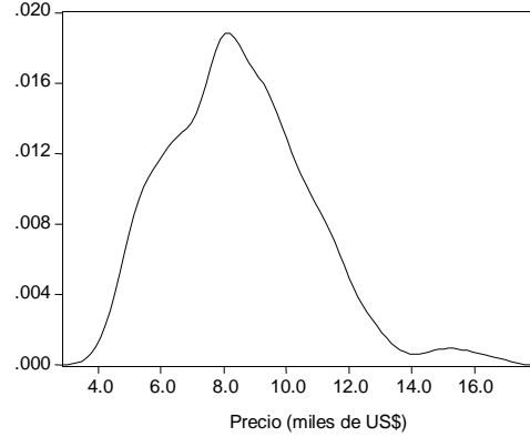
Kernel Density (Normal, h = 5.1935 )
