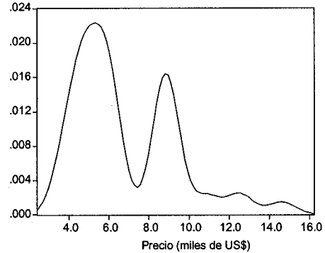
Kernel Density (Normal, h = 2.7217 )
