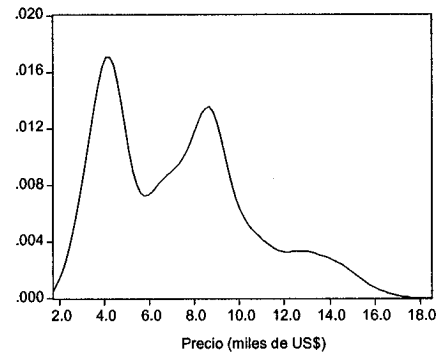
Kernel Density (Normal, h = 6.7804 )
