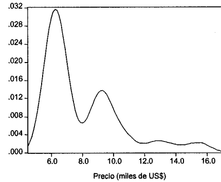
Kernel Density (Normal, h = 7.0822 )
