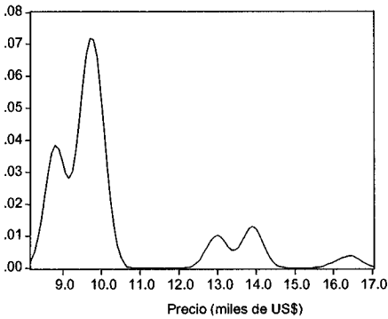
Kernel Density (Normal, h = 1.2433 )
