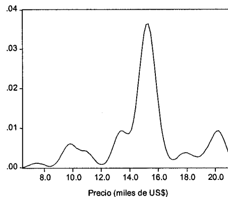
Kernel Density (Normal, h = 4.9394 )
