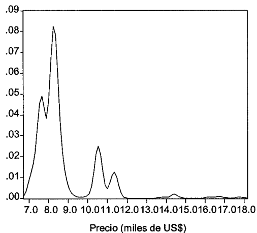
México Kernel Density (Normal, h = 1.7853 )
